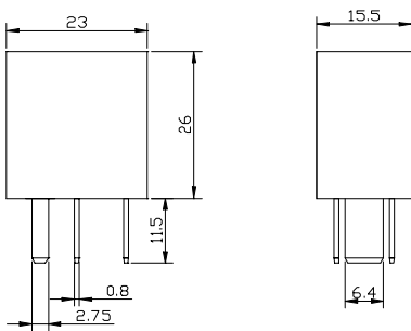
FRC7 - Plug in type with 2.75mm pin width for pins#85 & #86
