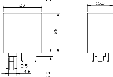
FRC7 - PCB type
