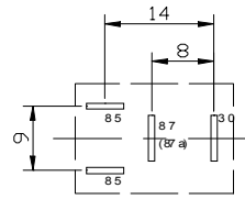
Plug in type
