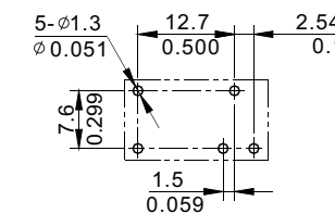
Mounting (Bottom view)
